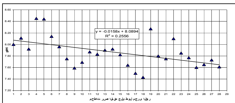
Figure 1: The development of the pH in Alassi River water..
