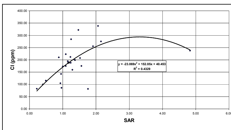
Figure 8: The relation between the Chloride and the Sodium Adsorbed Rate in Alassi River water
