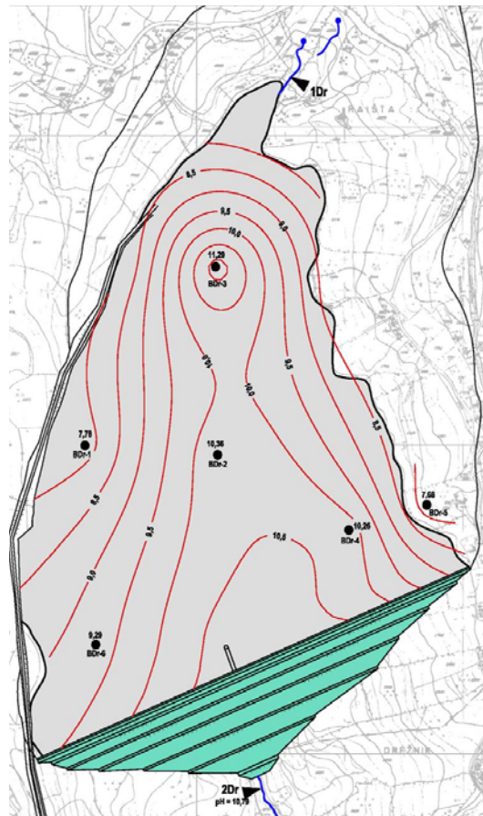
Figure 3b: pH contour lines at the Dreznik disposal site
