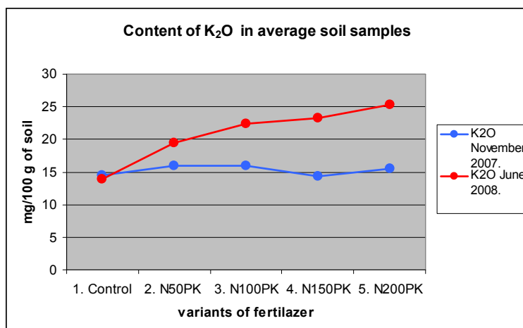
Figure 3: Content of K_2O in average soil samples
